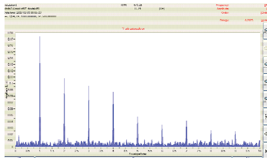
Fig. 5. Envelope order spectrum
