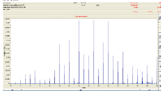
Fig. 3. Fourier spectrum of vibration signal of gas compressor
