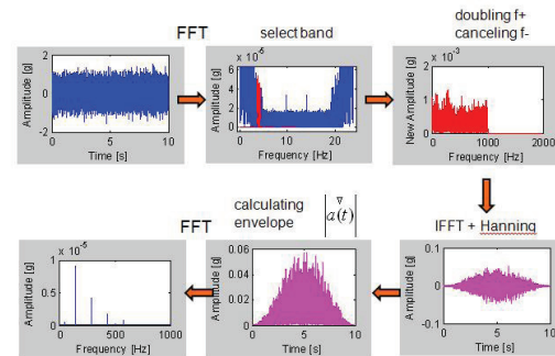
Fig. 7 The algorithm of envelope spectrum generation [1]
